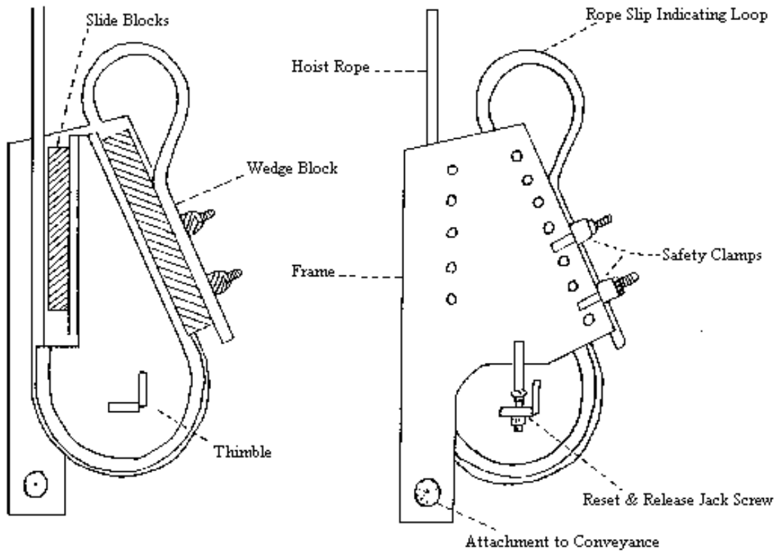
SHORT COUPLED THIMBLE
